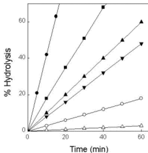
Fig. 3. Hydrolysis of ^{125}\text{I} -labeled Ub-PESTc by various DUBs. The same amount (0.1 \mu\text{g} ) of the purified YUH1 (○), yUBP6 (Δ), cUCH-1 (▼), cUCH-6 (●), cUCH-8 (▲), or cUBP41 (■) was incubated with 20 \mu\text{g} of ^{125}\text{I} -Ub-PESTc at 37 °C for various periods. After incubation, the release of PESTc was determined as described under Materials and Methods.
